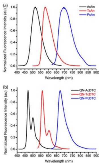
Figure 3. Normalized fluorescence spectra of (a) aniline-linked acenes and (b) dithiocarbamate-linked acenes in dichloromethane.
