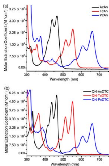
Figure 2. UV-vis absorbance spectra of (a) aniline-linked acenes and (b) dithiocarbamate-linked acenes in dichloromethane.
