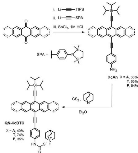
Scheme 1. Synthesis of the Unsymmetric Aniline- and Dithiocarbamate-Linked Diethynylacenes
