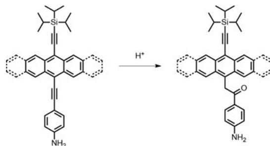
Scheme 2. Undesired Hydrolyzation of Aniline-Linked Acenes under Acidic Conditions
