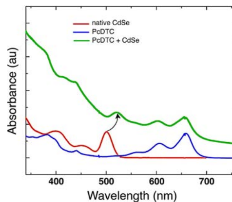
Figure 4. Absorbance spectra of PcDTC-capped CdSe QDs after 24 h of ligand exchange with QN-PcDTC in \text{CH}_2\text{Cl}_2 followed by serial precipitation and washing.
