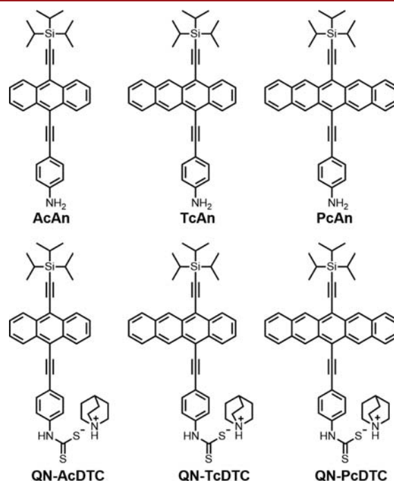
Figure 1. Structures of the acene ligands reported in this paper.
